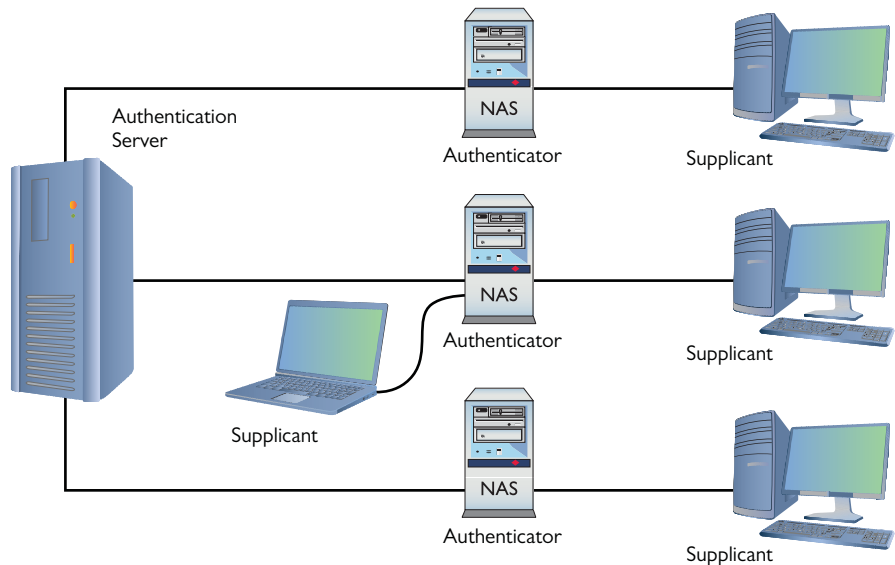
Figure 11-30 802.1X components
