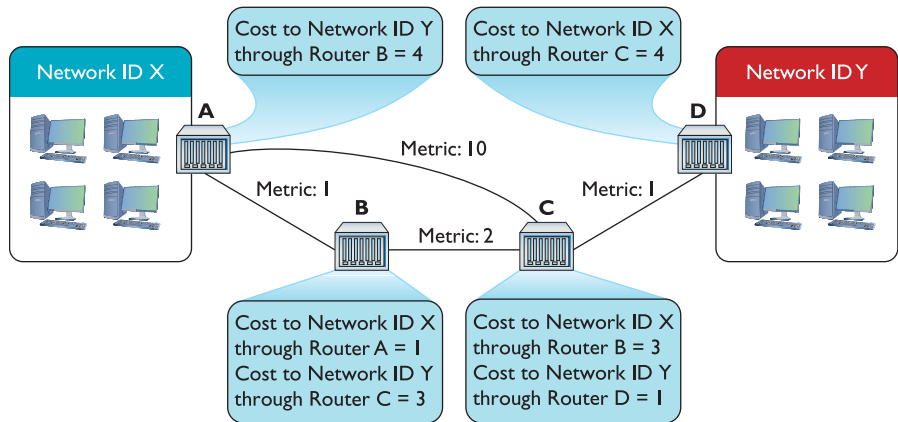
Figure 8-27 Last iteration
