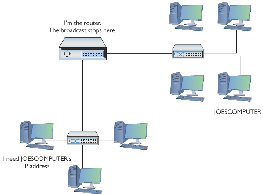
Figure 10-14 Routers don't forward broadcasts!
