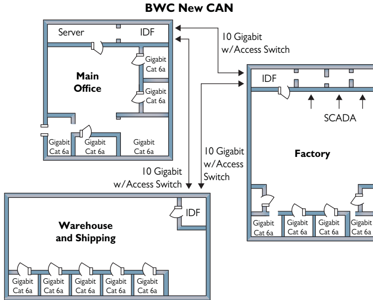
Figure 17-3 Connecting the buildings
