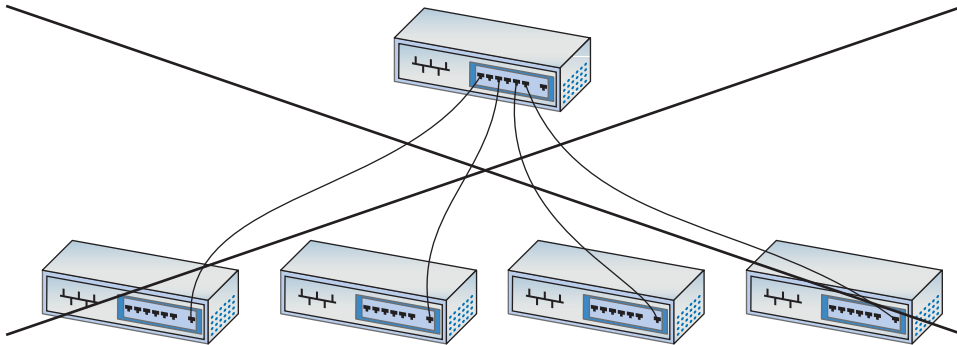
Figure 4-21 A hierarchical hub configuration will not work!
