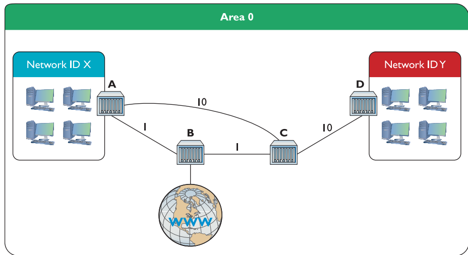
Figure 8-33 Area defined
