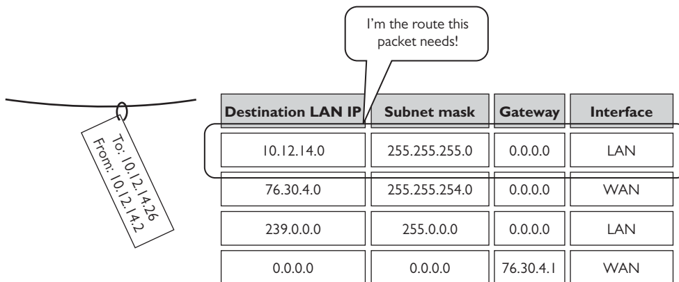
Figure 8-8 Routing table showing the route for a packet
