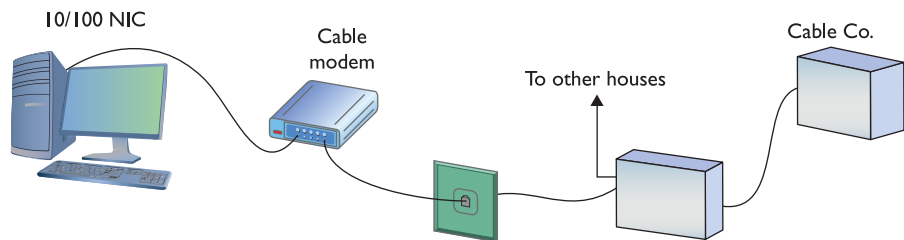
Figure 14-30 Cable modem
