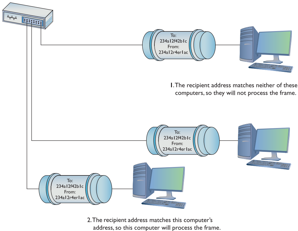
Figure 2-19 Incoming frame!
