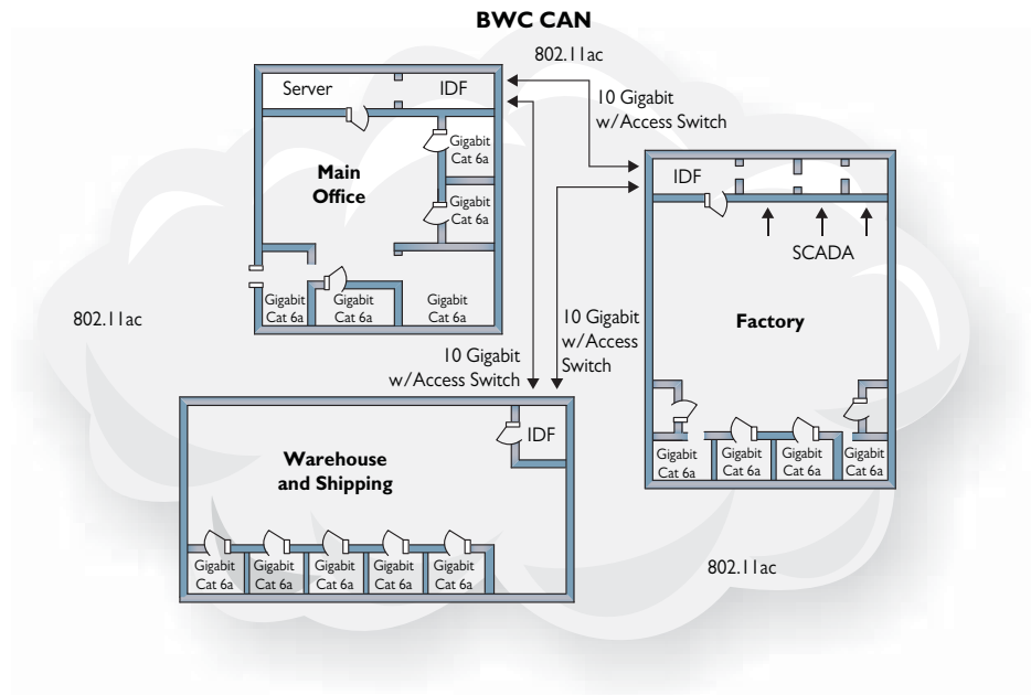
Figure 20-13 Diagram of Bayland Widgets' campus area network
