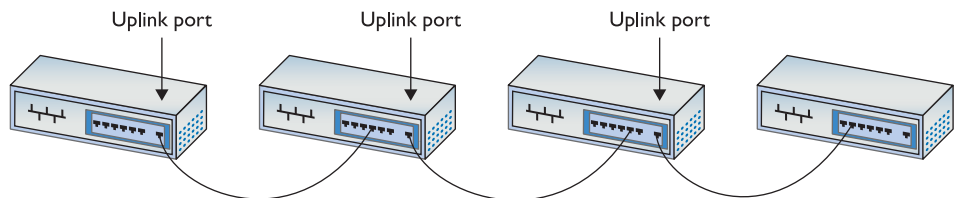
Figure 4-20 Daisy-chained hubs
