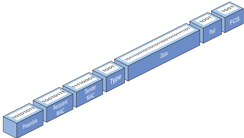
Figure 4-2 Ethernet frame
