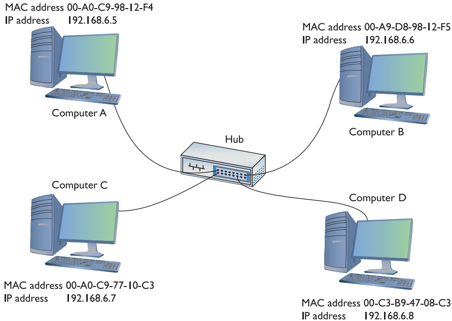
Figure 2-28 MHTechEd addressing
