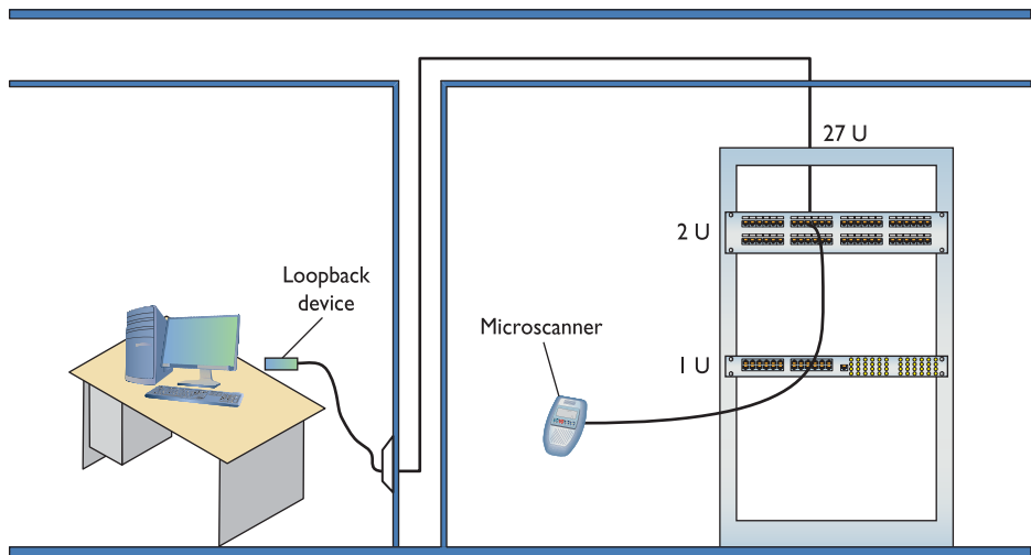
Figure 6-66 Loopback plug in action
