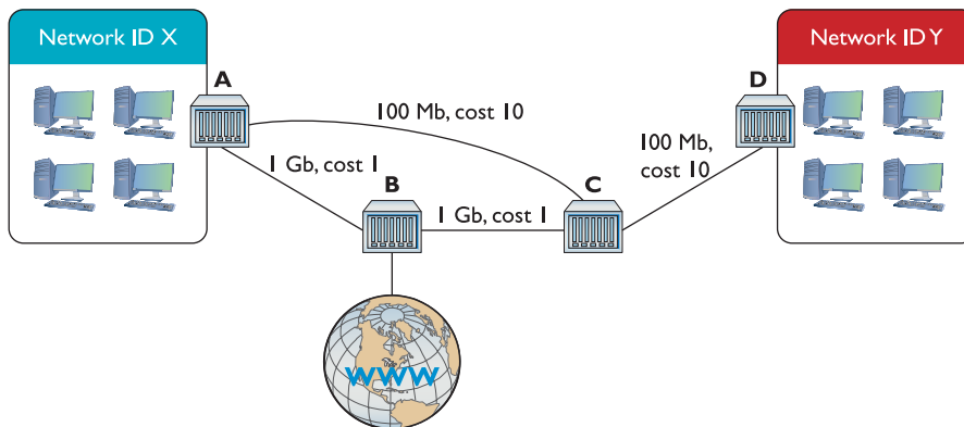
Figure 8-32 Link states
