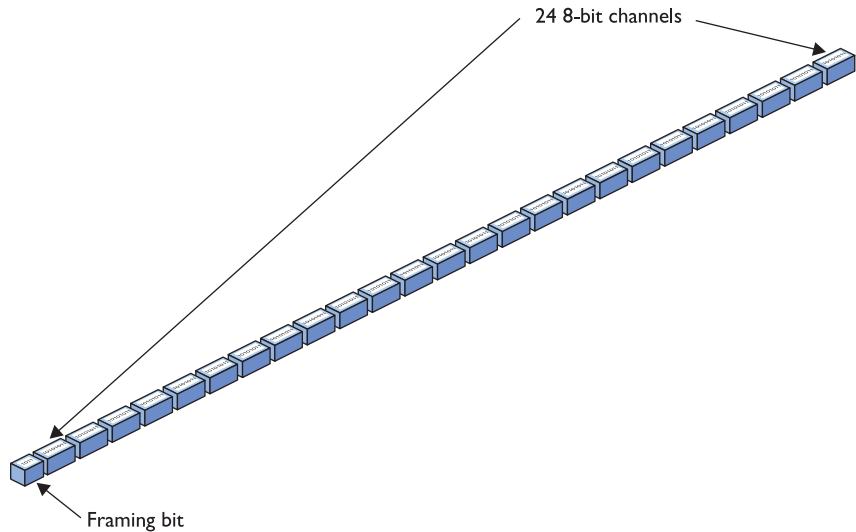
Figure 14-13 DS1 frame
