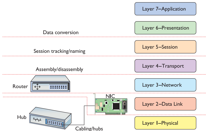
Figure 2-38 OSI updated
