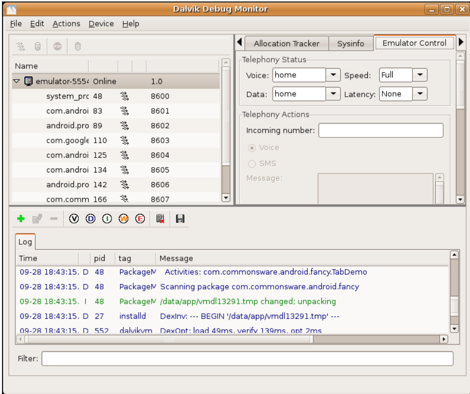
Figure 172. DDMS, with emulator selected
