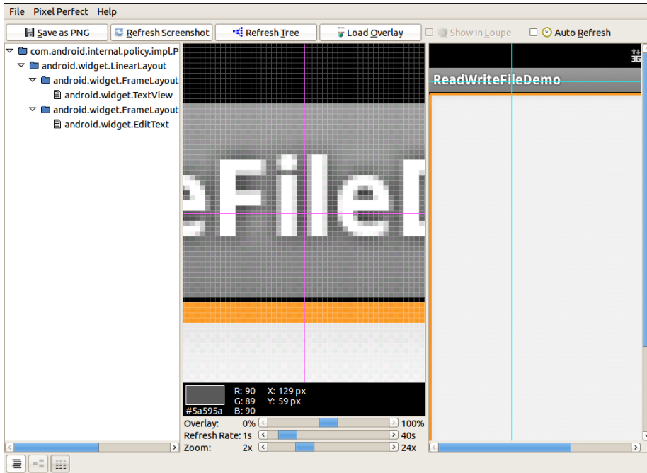
Figure 170. Hierarchy Viewer Pixel Perfect View
