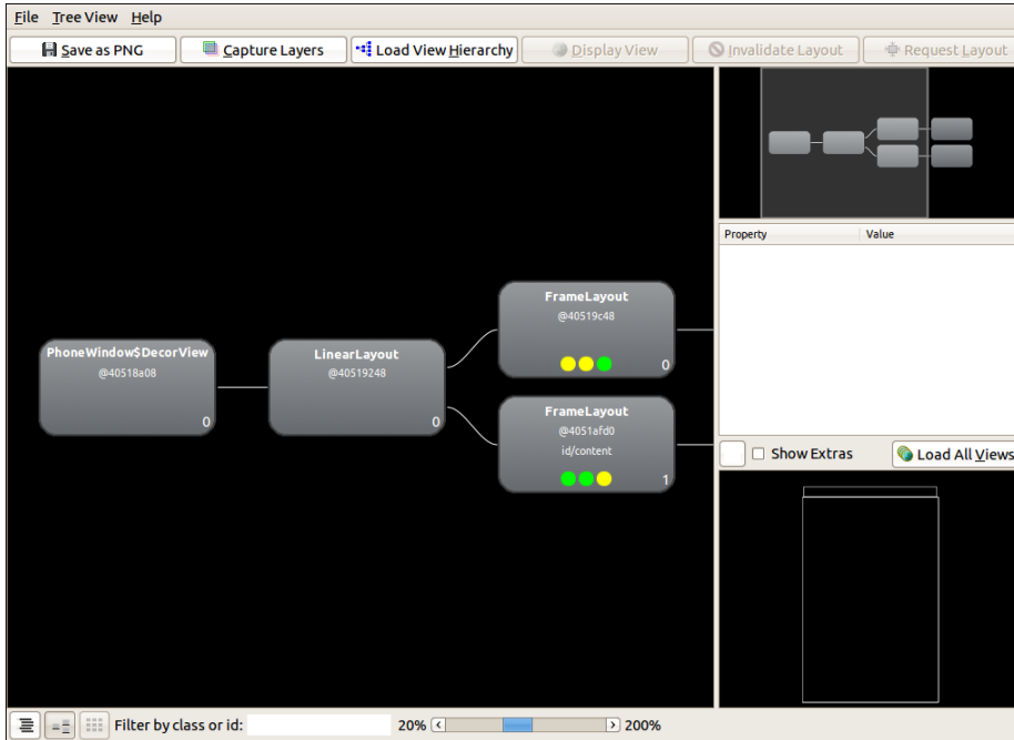
Figure 168. Hierarchy Viewer Layout View
