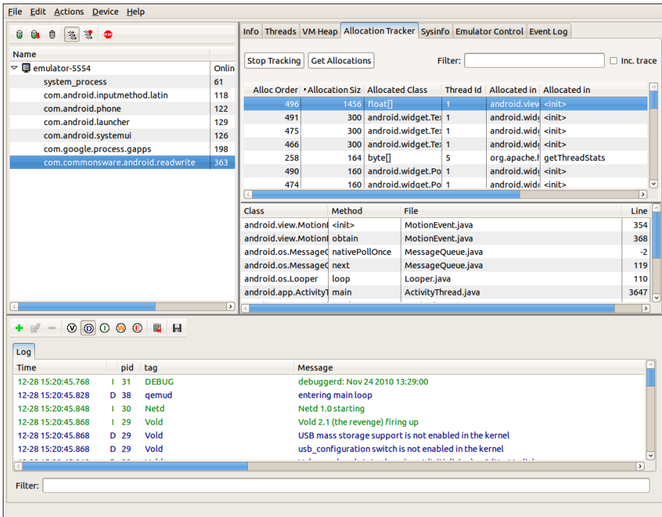
Figure 182. DDMS allocation tracker
