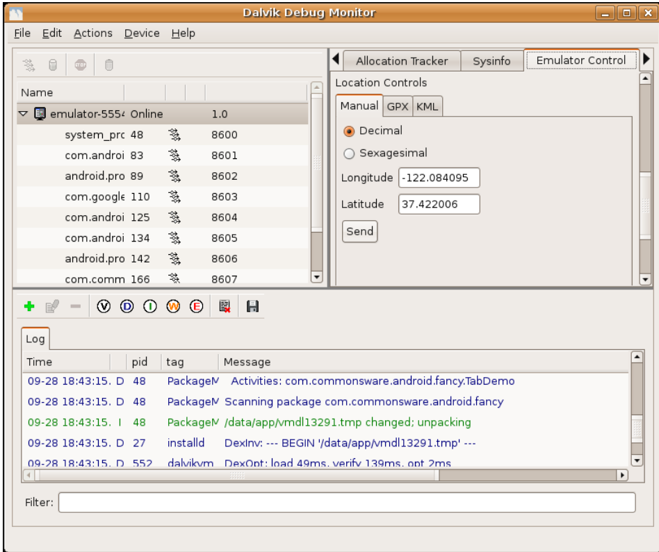
Figure 176. DDMS location controls
