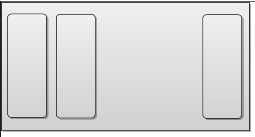
Figure 38. A LinearLayout with three children, with the third one right-aligned
