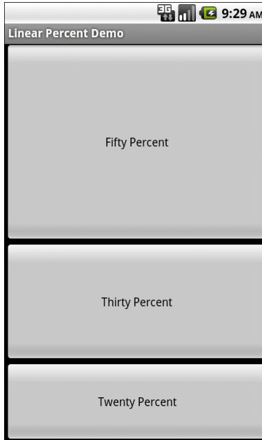
Figure 43. A LinearLayout split among three Buttons by percentage
