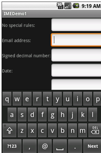
Figure 50. The input method editor for email addresses
