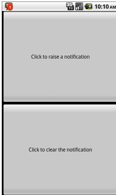
Figure 155. Our notification with the superimposed number
