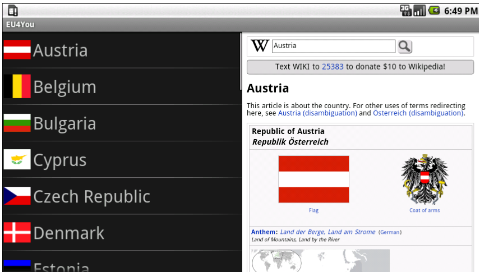
Figure 115. EU4You, landscape WVGA (800x480 pixels), set for normal density, and showing the embedded WebView
