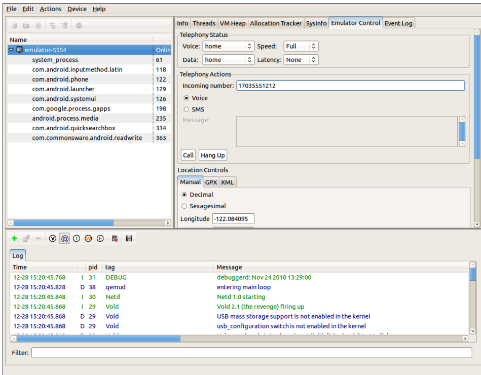
Figure 177. DDMS telephony controls
