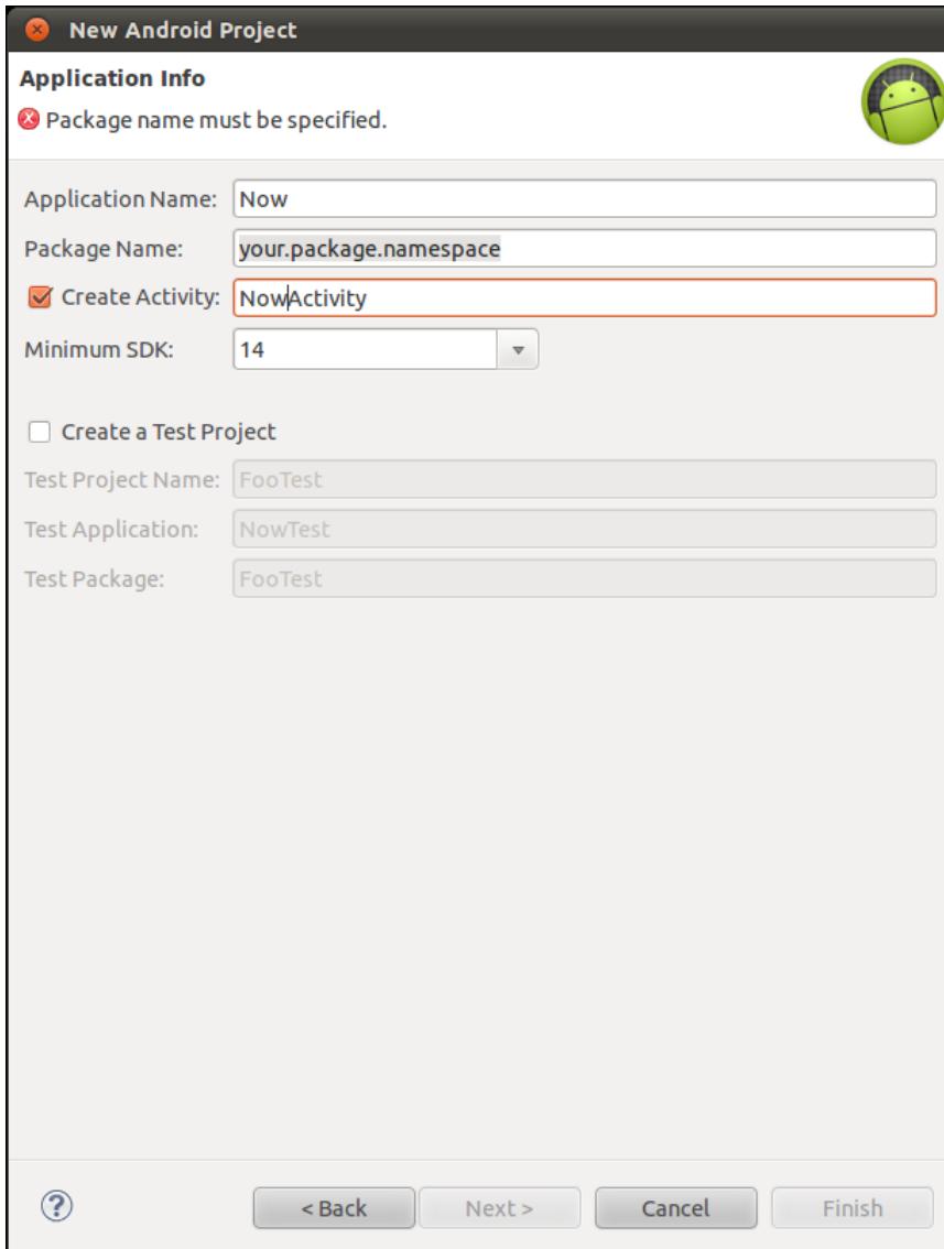
Figure 14. Eclipse New Project Wizard, Android Project (continued)
