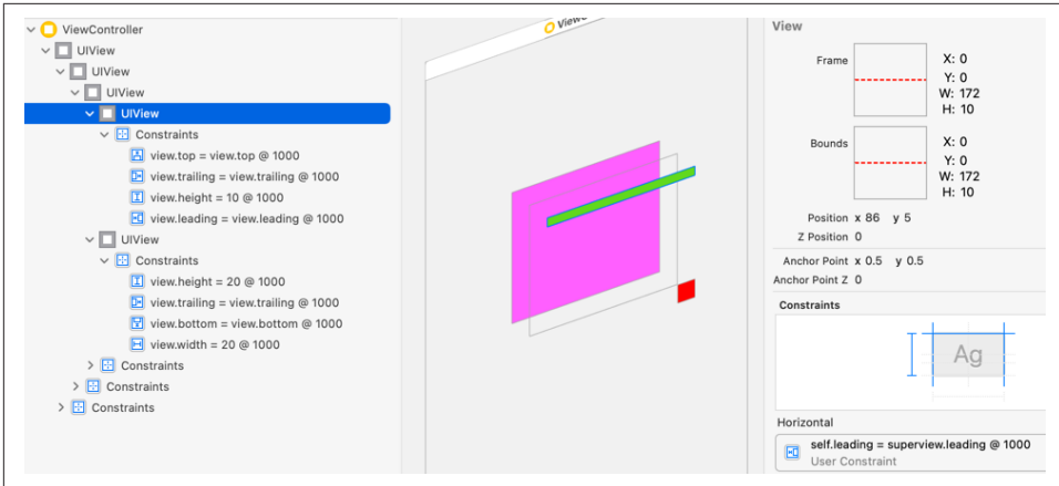
Figure 1-23. View debugging (again)
