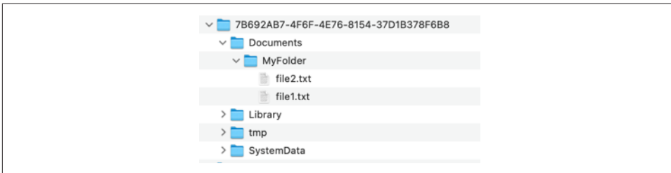
Figure 23-1. An app's sandbox in the Simulator
