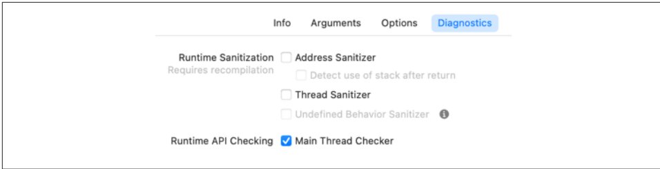
Figure 25-1. The Main Thread Checker is watching you
