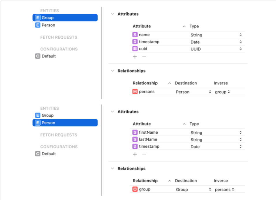
Figure 23-11. The Core Data model for the People Groups app
