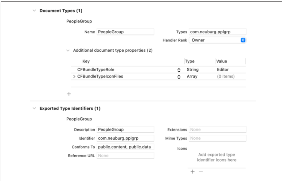
Figure 23-8. Defining a custom UTI
