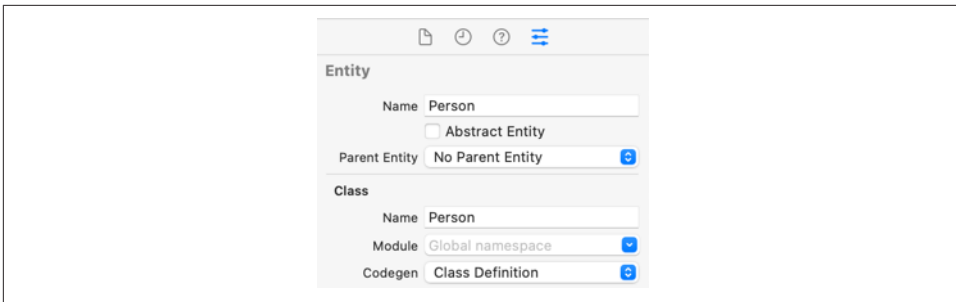
Figure 23-12. Configuring code generation
