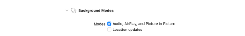
Figure 15-2. Using Capabilities to enable background audio
