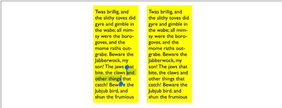
Figure 11-18. A text storage with two layout managers
