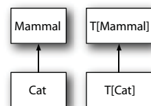
Figure 6.2 Covariance
