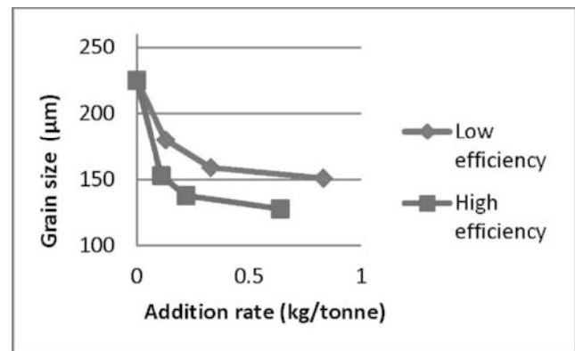
Figure 1. Grain refiner curves for two master alloys with different efficiency.
