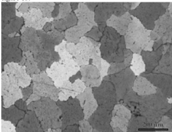
Figure 13. Billet micrograph of heat 5407B. Optifine was added at 0.65 kg/t. Titanium 0.005%. Grain size 110 \mu\text{m} .
