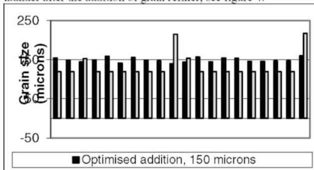
Figure 4. Grain sizes after optimized additions compared with estimated grain sizes, in absence of optimization.
