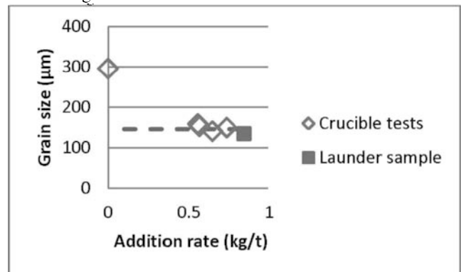
Figure 11. Grain sizes in crucible test samples and launder sample at an addition rate of 0.85 kg/t, charge 5404B. The horizontal line indicates the predicted grain size for charges with a level of Ti adjusted to 50 ppm in the casting furnace.
