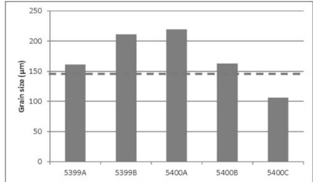
Figure 10. Grain sizes in Opticast samples collected at casting table for 5 charges cast with an addition rate of 1.1 kg/t. The horizontal line indicates the predicted grain size for charges with a level of Ti adjusted to 50 ppm in the casting furnace.
