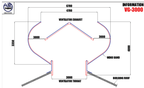
Figure 2 Configuration of Tulip shape ventilator
