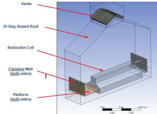
Figure 1. General Layout of Reduction Cell in Building
