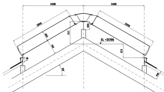
Figure 3 Configuration of Low Profile shape ventilator
