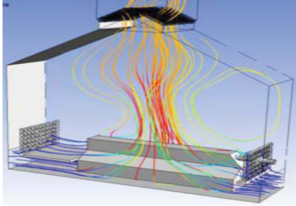
Figure 4 Low Profile Simulation
