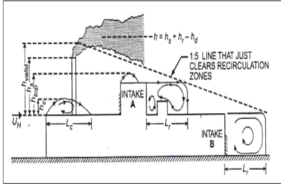
Figure 8 Flow Recirculation ASHRAE 2003
