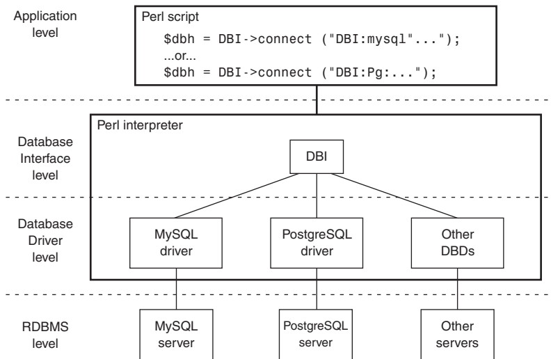
Figure 6.1 DBI architecture.
