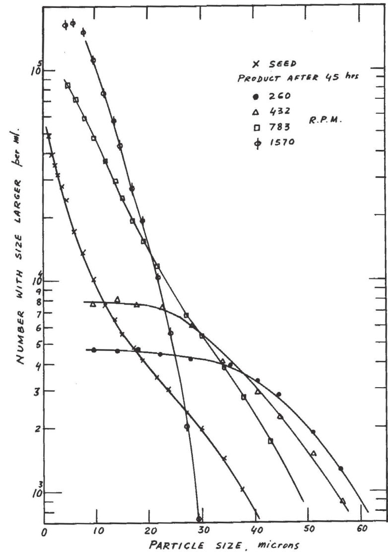
Fig. -2 Change in size distribution due to agglomeration and growth.
