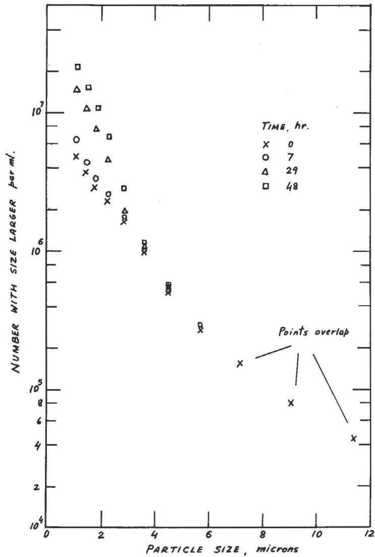
Fig.-7 Generation of small particles by attrition.
