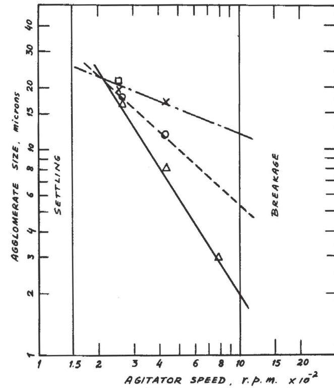
Fig.-4 Dependence of agglomerate size on agitator speed.
