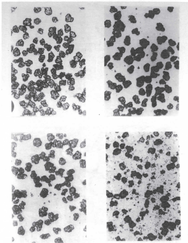
Fig. -5 Gross breakage of coarse seed at high agitator power input.
