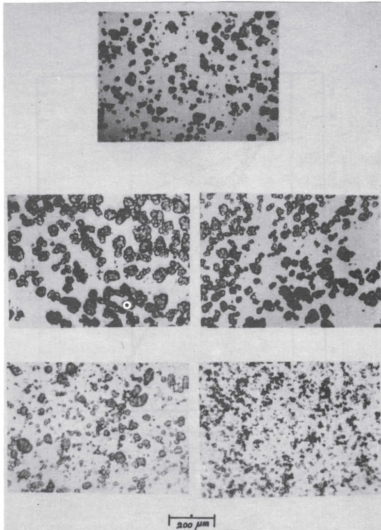
Fig.-3 Effect of increased agitator power input on precipitation from fine seed of mixed particle size distribution.
