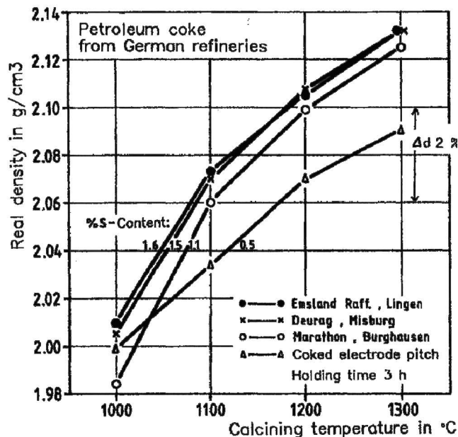
Figure 5: Increase in real density of petroleum coke with the heat-treatment temperature
