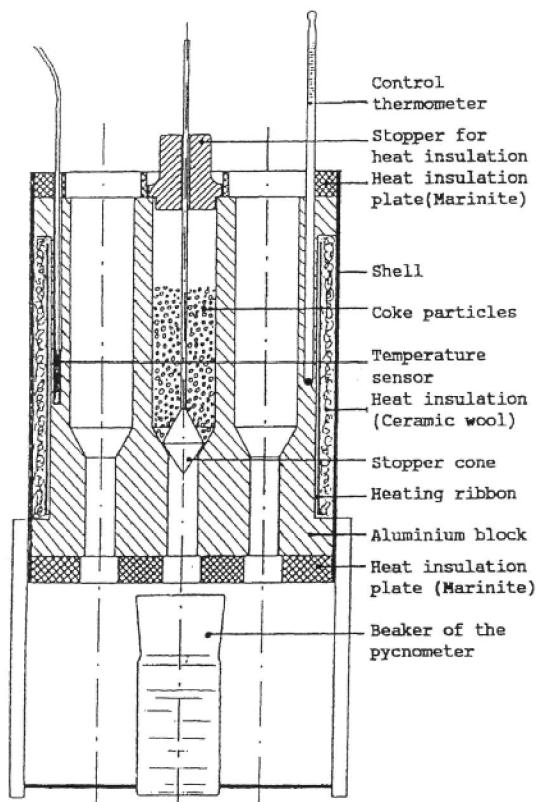
Figure 3: Vertical section of the preheating apparatus for the AD determination of carbon particles by means of the water method
