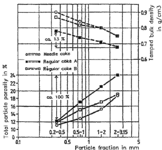
Figure 6: Comparison of the tamped bulk density and total particle porosity of petroleum coke
