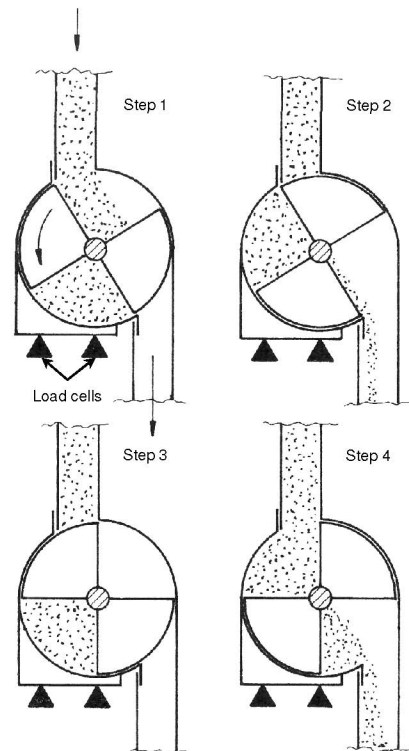
Figure 9: Cellular wheel feeder for the volumetric proportioning of particle fractions combined with weight control
