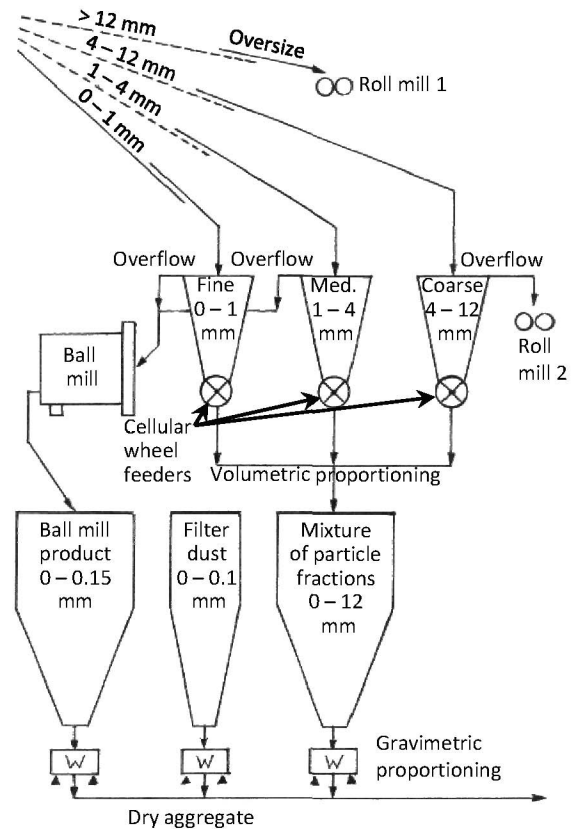
Figure 8: Volumetric proportioning of the granular particle fractions in the paste plant
