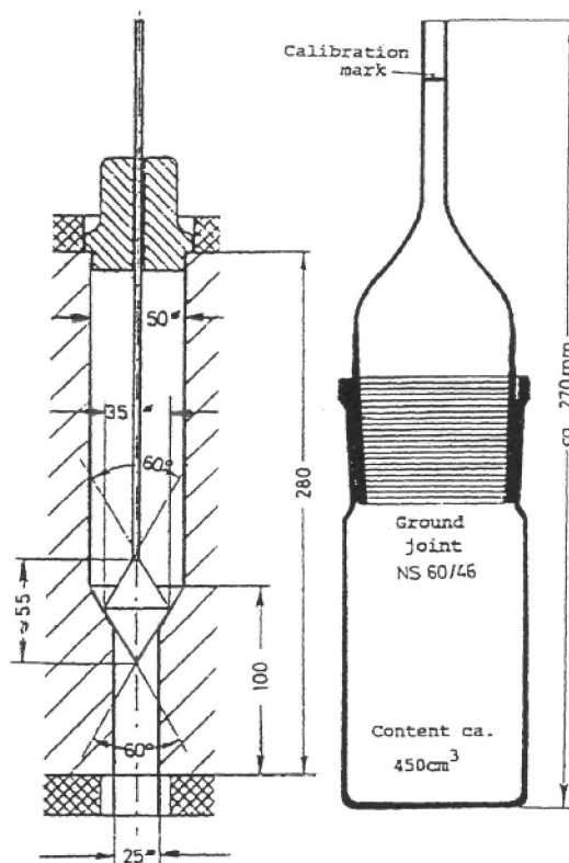
Figure 4: Heating-cell dimensions and pycnometer for the AD determination of carbon particles by means of the water method
