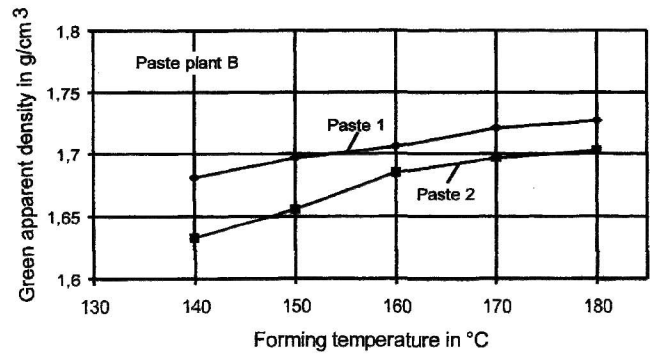
Figure 11: Anode paste compaction as a function of temperature
