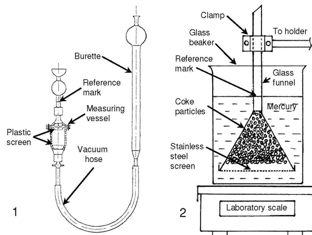
Figure 1: Mercury volumenometer for determining the AD of granular material (DIN 51065, page 2, 1964)
