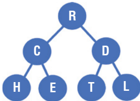
Figure 15.6: Swapping D and T is the first step to balance this heap.
