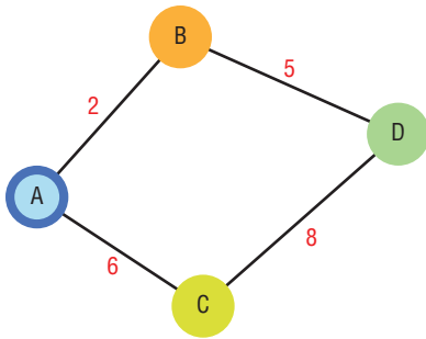
Figure 16.11: A graph with four vertices
