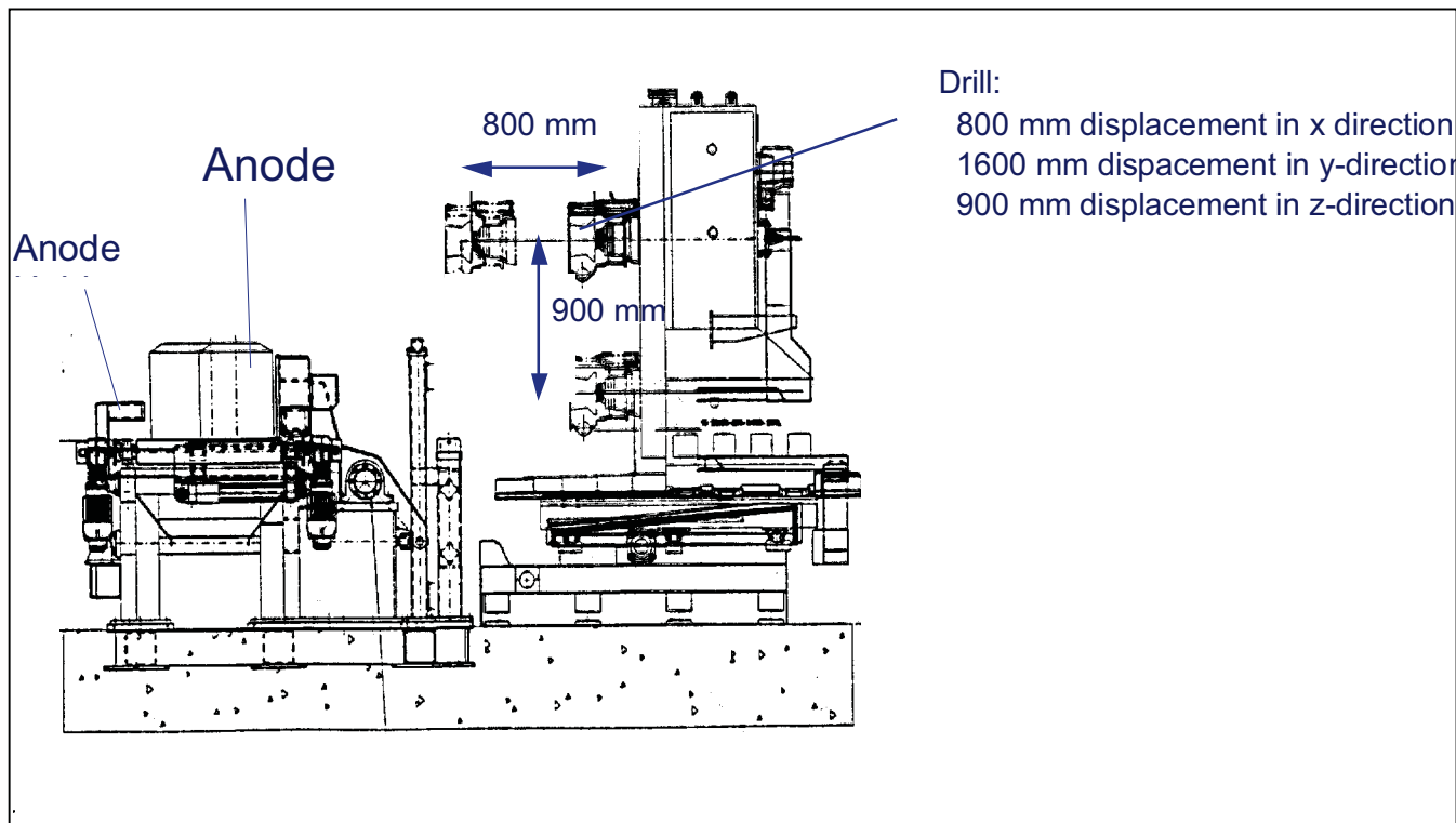
Figure 1: Stub hole drilling machine.
