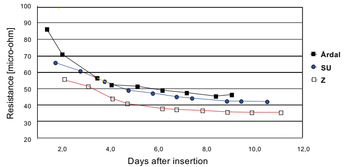
Figure 5. Measured resistance between stub and anode, with the different stub hole designs, as a function of time after insertion.
