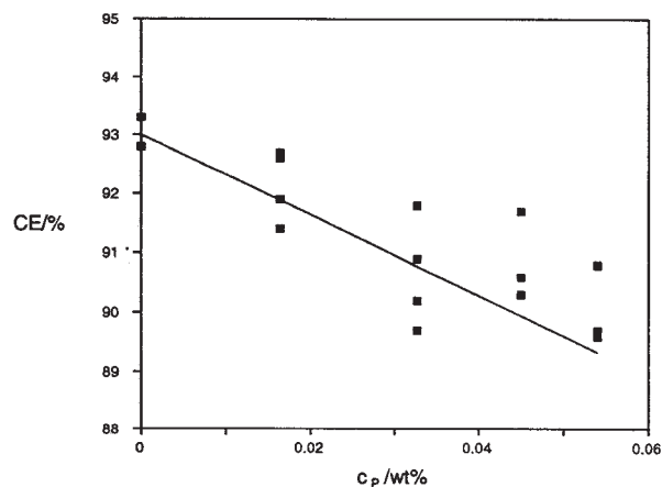
Fig. 16: CE as a function of the total electrolyte concentration of phosphorous cations. Regression line: CE = (93.0±0.5) - (67.8±18.4)c P .
