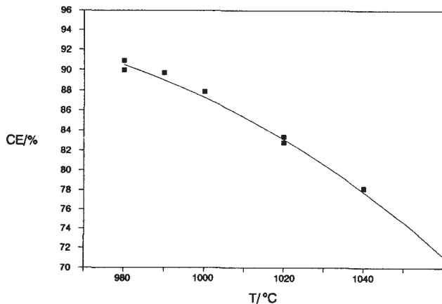
Fig. 8: CE as a function of temperature at r = 3.0 . Points: experimental values. Line: CE model. Cathodic current density 0.85 \text{ A/cm}^2 , 5 wt% \text{CaF}_2 , and 4 wt% alumina.
