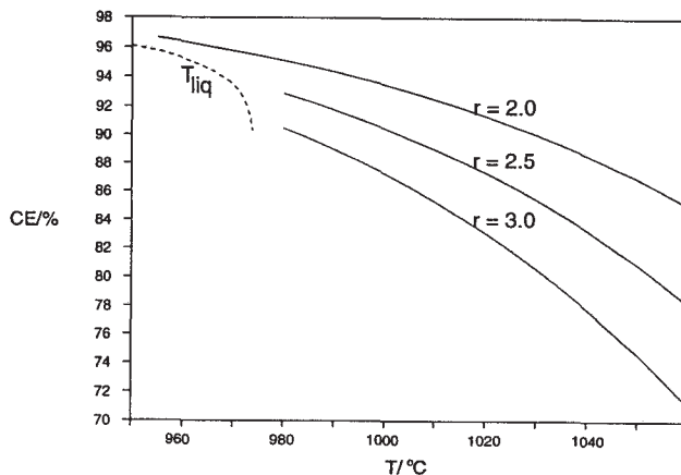
Fig. 9: CE as a function of temperature ( T ), model lines for cryolite ratios 2.0, 2.5 and 3.0. The liquidus temperature is indicated by the dotted line.
