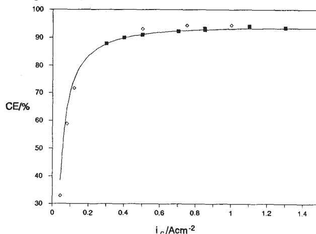
Fig. 3: CE as a function of cathodic current density, i_c . Temperature 980°C, NaF/ AlF_3 ratio 2.5, 5 wt% CaF_2 and 4 wt% alumina. Filled squares: present work, diamonds: Skybakmoen and Sterten 7 , solid line: CE model.
