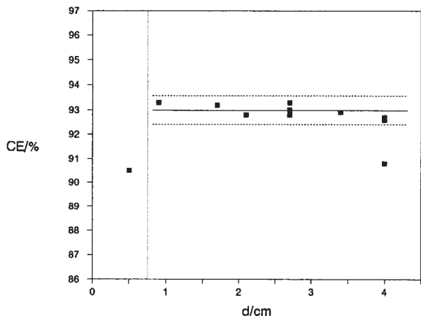
Fig. 4: CE as a function of inter-polar distance (d). Temperature 980°C, NaF/AlF 3 ratio 2.5, 5 wt% CaF 2 , 4 wt% alumina and cathodic current density 0.85 A/cm 2 . The approximate critical anode-cathode distance is indicated by the dotted vertical line.
