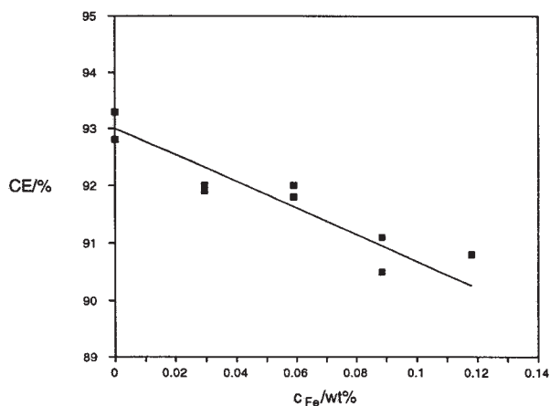
Fig. 15: CE as a function of the total electrolyte concentration of iron cations. Regression line: CE = (93.0±0.5) - (23.2±3.8)c Fe .
