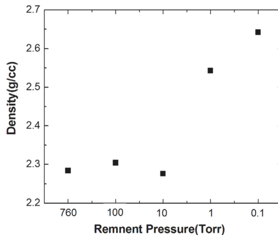
Figure 5: The measured densities of the RPT specimen as a function of remnant pressure. The melts were held at reduced pressure for 30 minutes before RPT.
