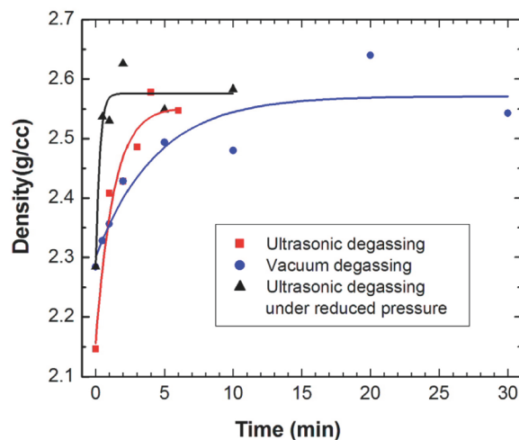
Fig. 8: The efficiency of different degassing techniques when remnant pressure is 1 Torr. The techniques include ultrasonic degassing, vacuum degassing and ultrasonic degassing under reduced pressure.
