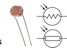
LDR with Schematic Symbol
