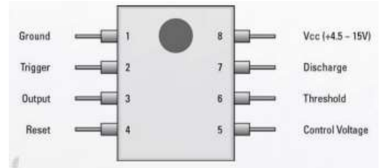
555 timer schematic diagram
