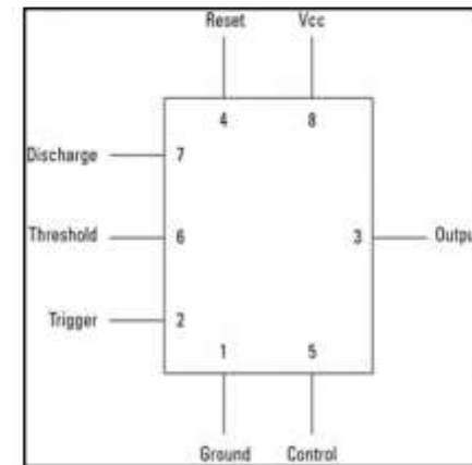
555 timer schematic diagram
