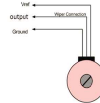
(B) Potentiometer terminals connections and schematic
