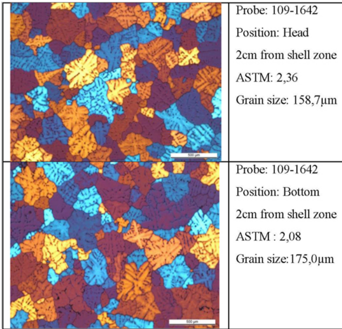
Figure 2. Grain size measurement - standard grain refiner
