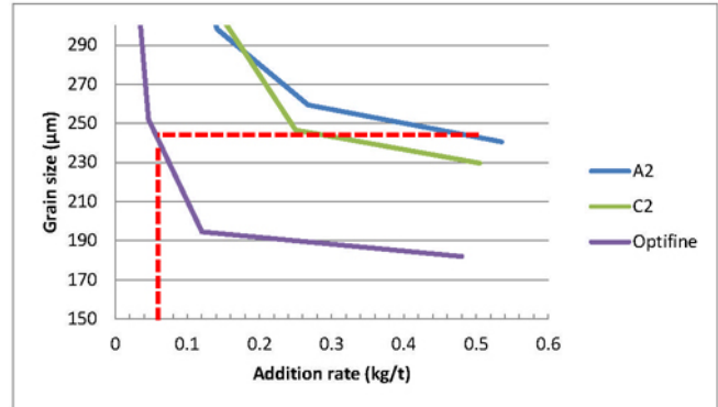
Figure 6. Results of crucible tests of different grain refiner samples in batch 109 - 1640
