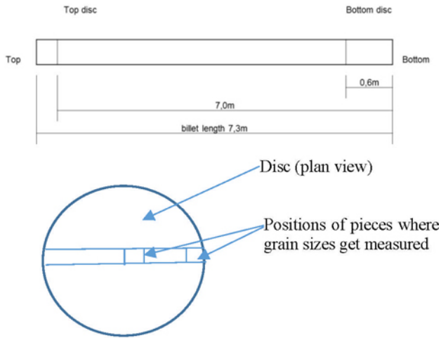
Figure 1. Position of sample discs cut from billets
