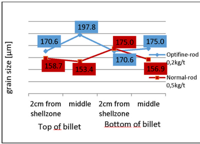
Figure 5. Chart of grain size measurements of disks
