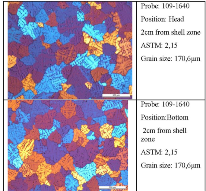
Figure 3. Grain size measurement - Optifine grain refiner
