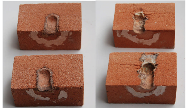
Figure 15: Results of vermiculite (left) and diatomite (right) insulating bricks corrosion test
