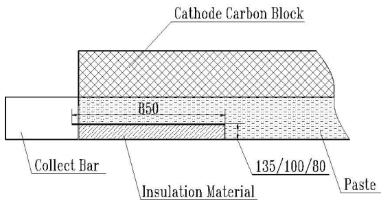
Figure 10: Partial paste ramming connection [2]
