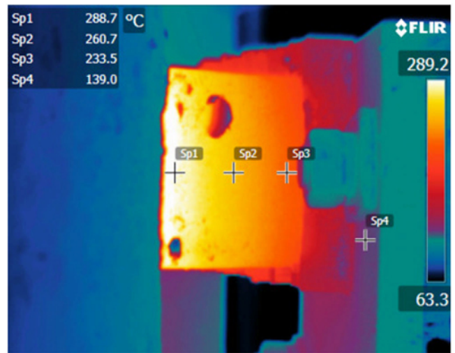
Figure 7: Infrared picture from thermal imager for steel collector bar
