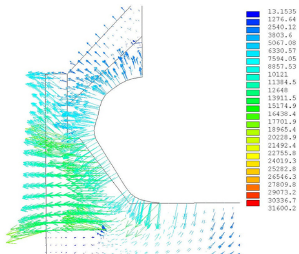
Figure 5: Heat flux of side ramming paste
