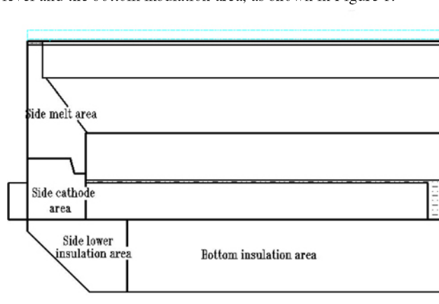
Figure 1: Pot lining zones [1]
