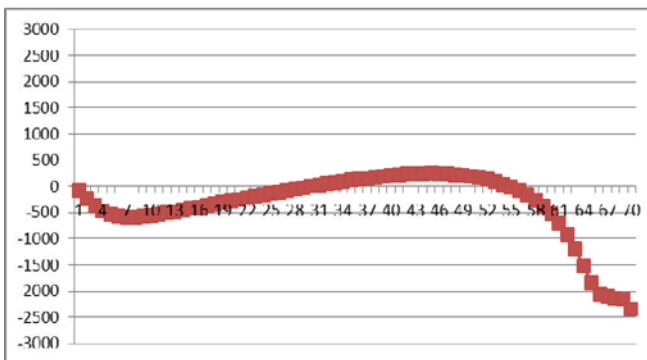
Figure 11: Curve Partial paste ramming connection (insulation height 80)
