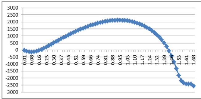
Figure 9: Metal pad horizontal current density for full ramming paste connection
