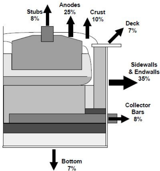
Figure 13: Typical heat loss partition of high amperage cell [3]
