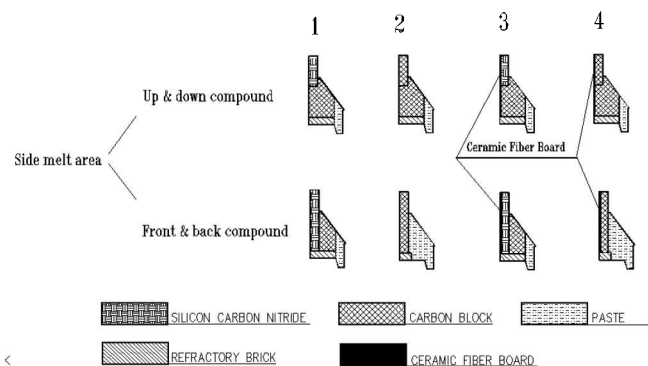
Figure 3: Side wall area at liquids level
