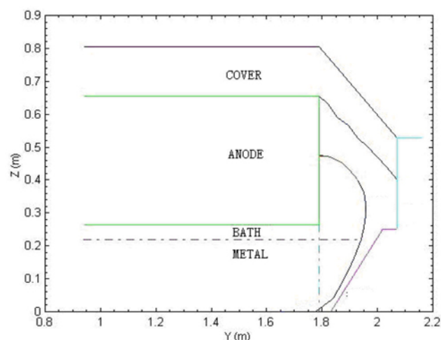
Figure 2: Optimum ledge profile
