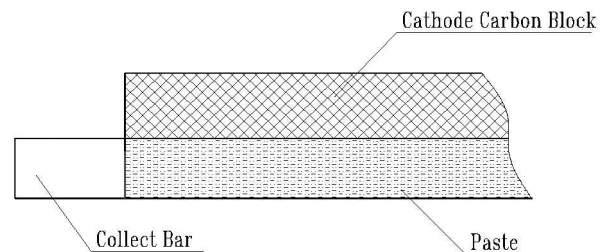
Figure 8: Full ramming paste connection
