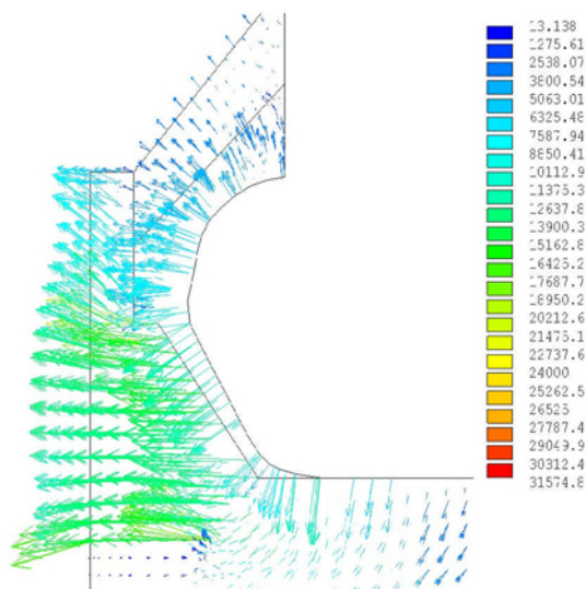
Figure 4: Heat flux of side profiled carbon block
