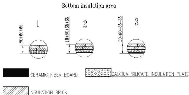
Figure 14: Bottom insulation area
