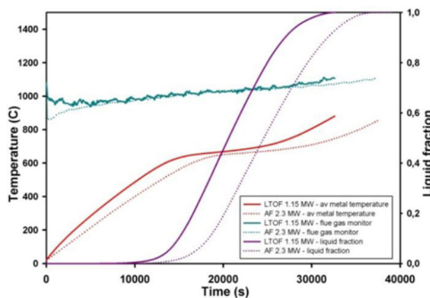
Figure 2: Furnace evaluation for melt pool configuration for 1.15 MW LTOF burner input and 2.3 MW air-fuel burner input [2].
