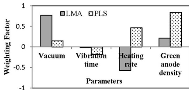
Figure 2. Effect of different parameters on baked anode density using LMA and PLS analyses.
