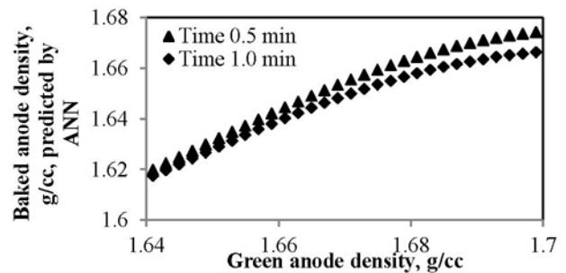
Figure 6. Effect of green anode density on baked anode density.
