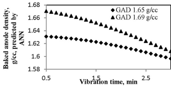
Figure 4. Effect of vibration time on baked anode density.
