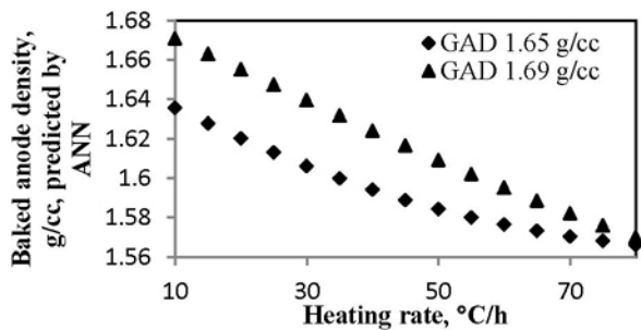
Figure 5. Effect of heating rate on baked anode density.
