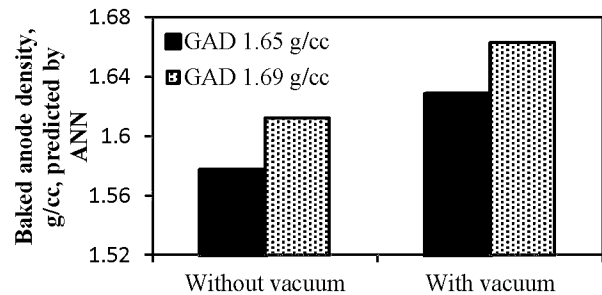
Figure 3. Effect of vacuum on baked anode density (GAD: Green Anode Density)
