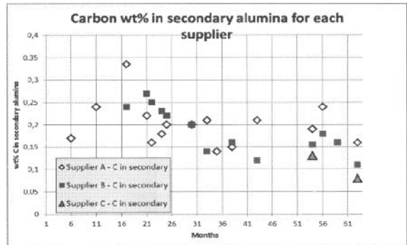
Figure 4: Carbon in secondary alumina of samples taken from Fume Treatment Plants dedicated to pot sections where the supplier anodes are used.
