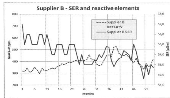
Figure 8: SER and reactive elements for supplier B.
