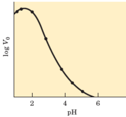
(a) Pepsin
