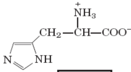
Histidine
