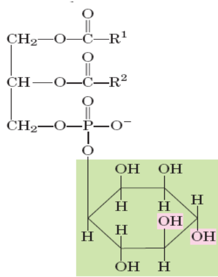
Phosphatidylinositol
