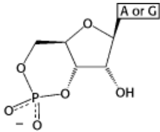
cAMP, cGMP
