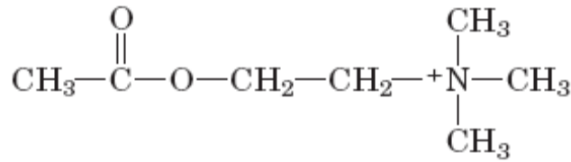
Acetylcholine
