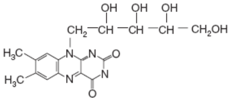
Riboflavin
