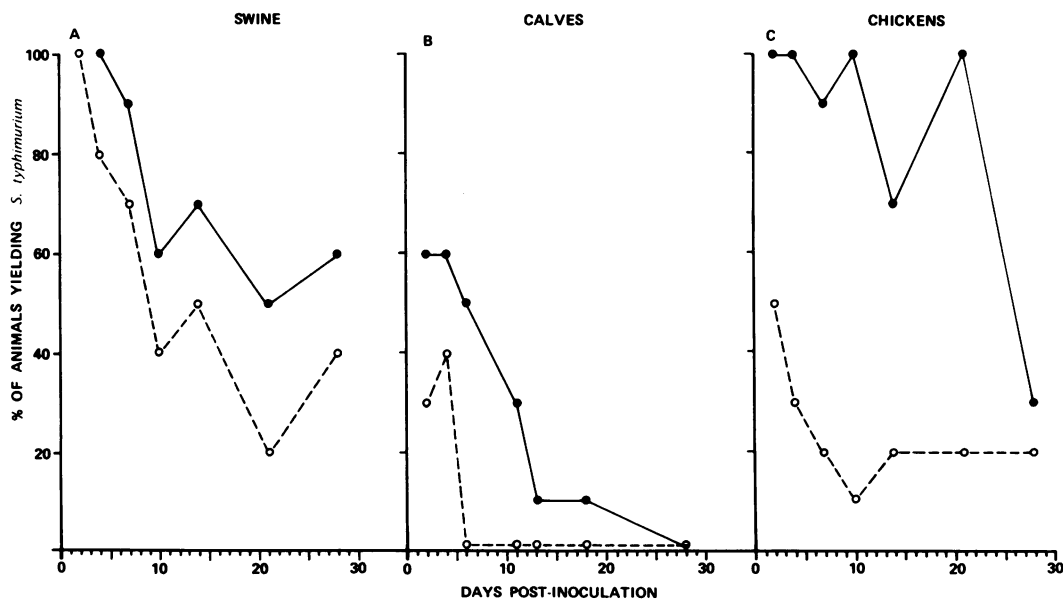
FIG. 1. Percentage of animals shedding S. typhimurium . Symbols: ●, nonmedicated controls; ○, oxytetracycline treated.
